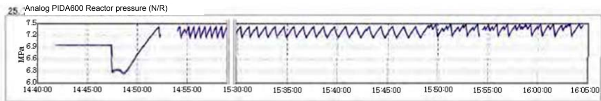
Fig. 2.1-3-3 Unit 3's reactor pressure (trend data by transient recorder)
