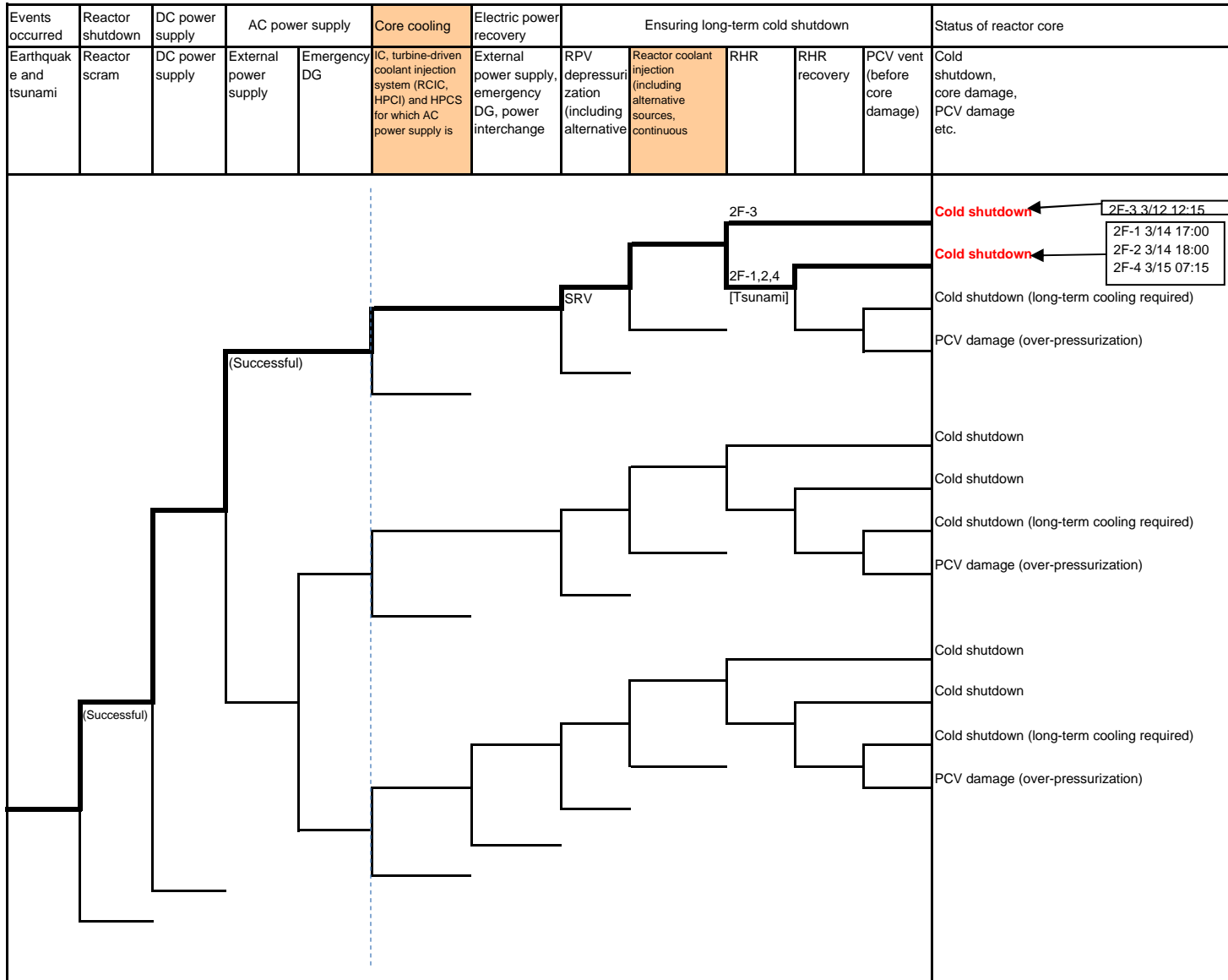
Figure Appendix 3-1 Fukushima Daini Nuclear Power Station disaster identification events tree
